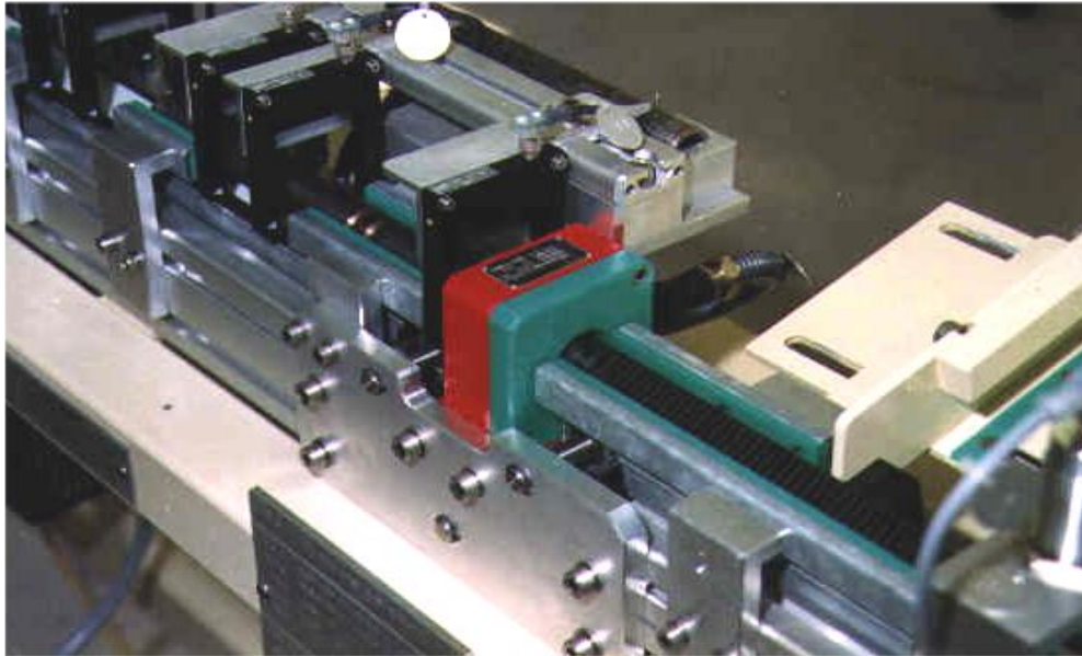
Test part in test position 4. Good view of test coil and fork type light barriers.
