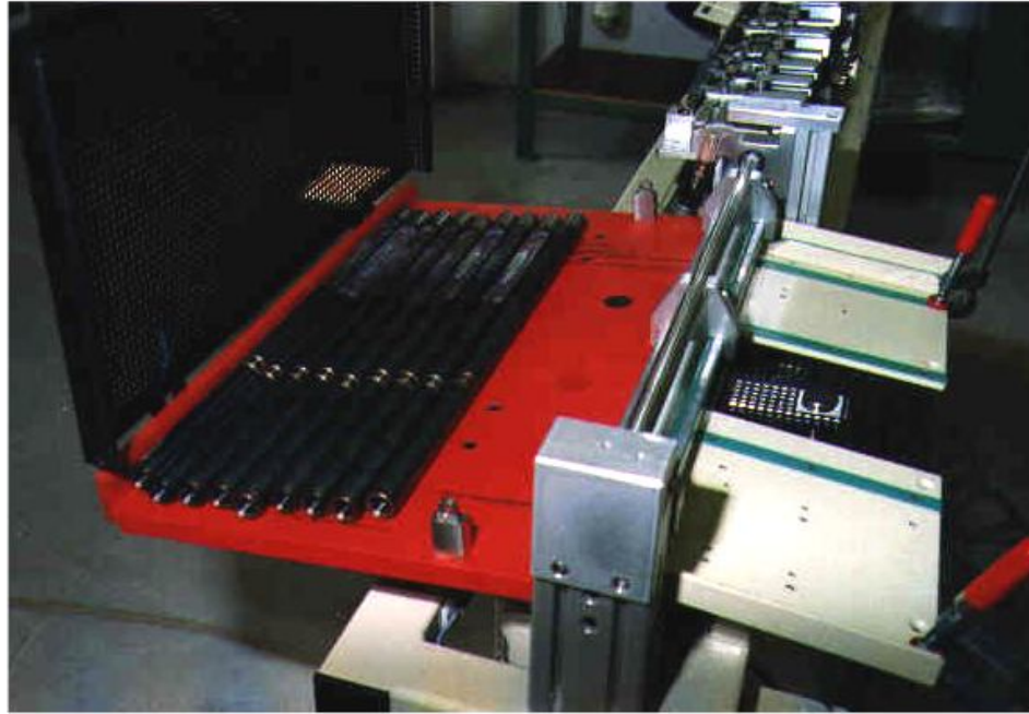
Discharge of parts to the left into a lockable rejected parts tray. O.K. parts are forwarded to the right.
