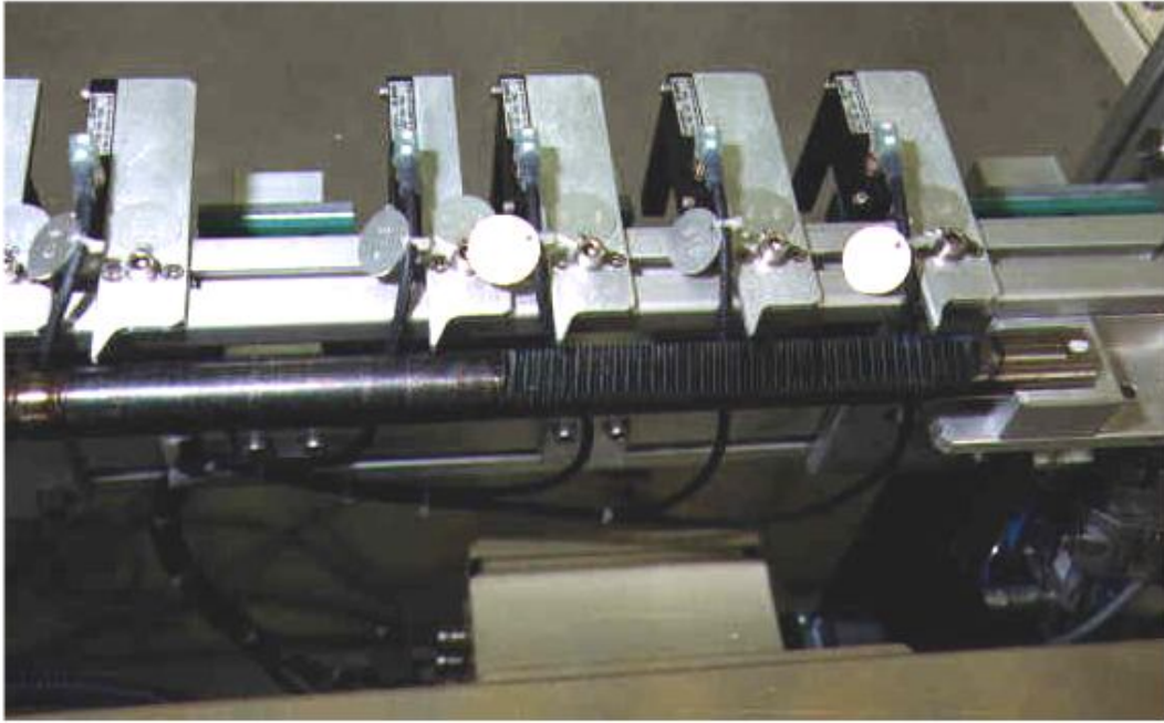
The test positions are adjusted by means of a master steering rack and adjustable light barriers. For this reason the system is very versatile and can easily be set for other parts types.
