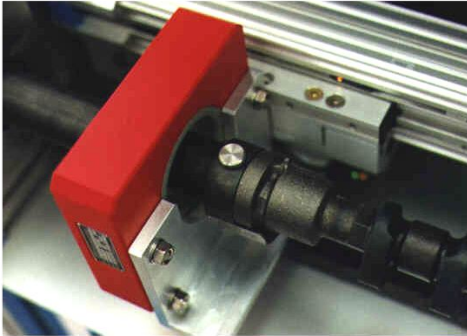
The test coil automatically moves to up to 16 programmable test positions.
